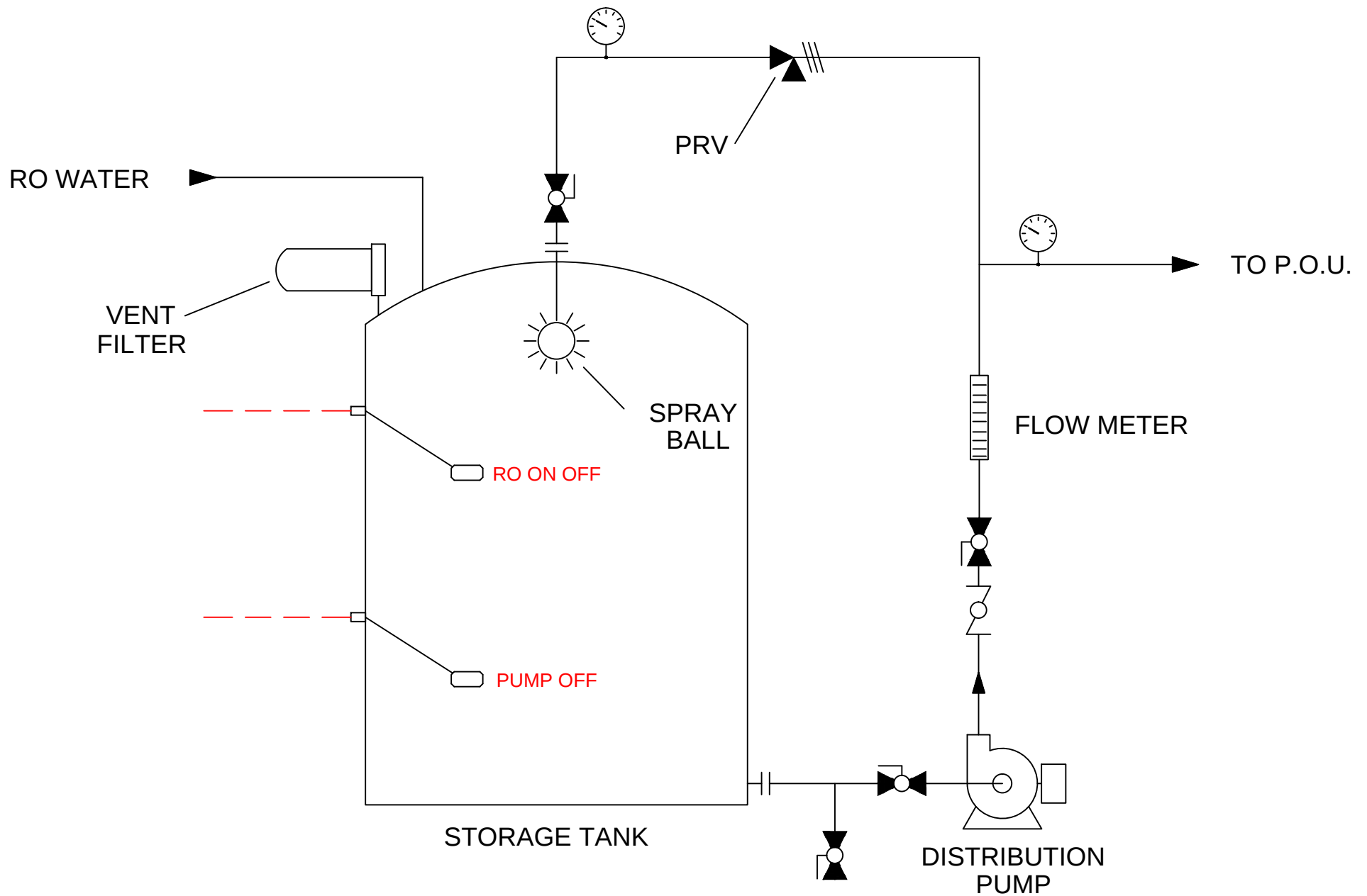
TANK RECIRC. SYSTEM
